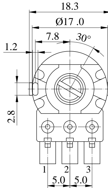
SHAFT SHOWN IN FULL C.C.W POSITION
