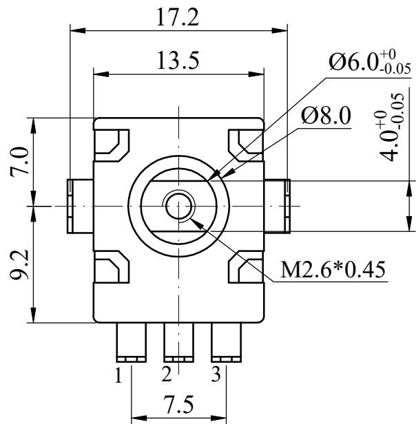
SHAFT SHOWN IN FULL C.C.W POSITION
