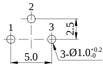
Mounting Hole
