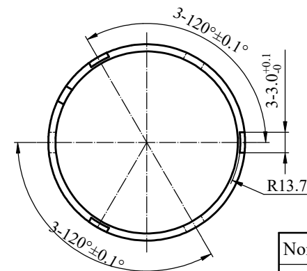
SHAFT DETAIL
