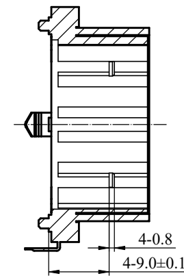
SECTION E-E
