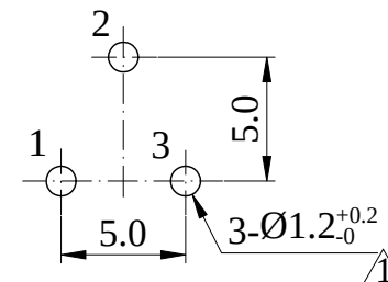
Mounting Hole
