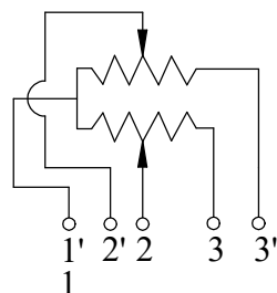
CIRCUIT
