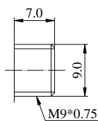
Bushing Dimension
