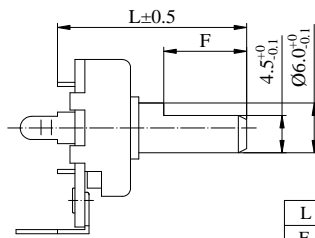
Bushing Dimension
