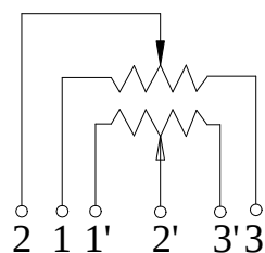
CIRCUIT
