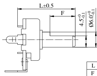
Bushing Dimension
