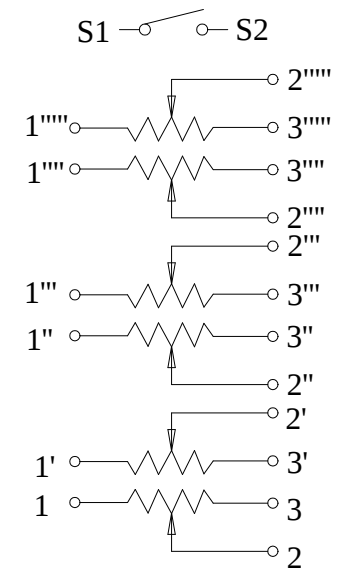
SHAFT SHOWN IN FULL C.C.W POSITION
