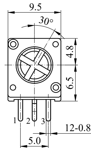
SHAFT SHOWN IN FULL C.C.W POSITION
