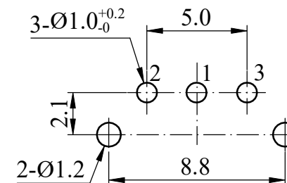
Mounting Hole
